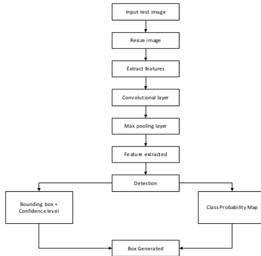
Fig. 8. Block diagram of dataset testing.
