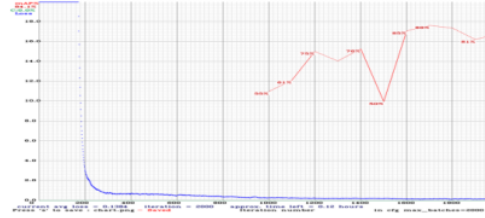
Fig. 10. Mean average precision dataset iteration 2000.
