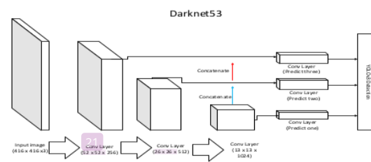
Fig. 1. YOLOv3 network architecture
